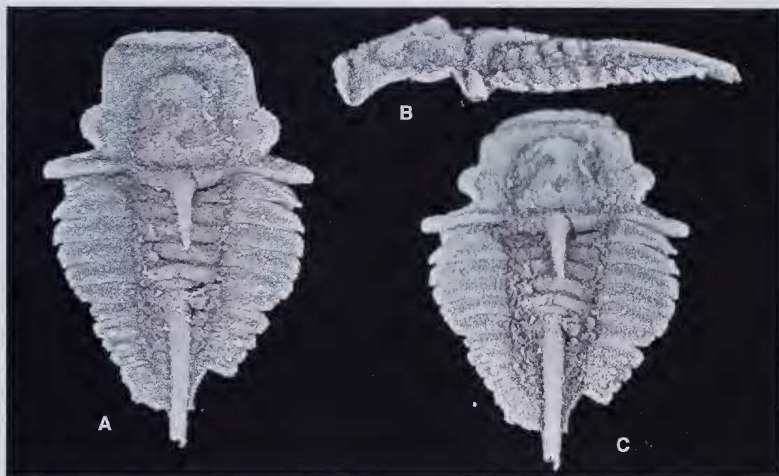
FIG. 11. Politicurus politus (Ross, 1951), from the Red Canyon Member, House Formation (Skullrockian, Bellefontia-Xenostegium Zone), Ibez area, section Lava Dam North 144.0m. A-C, articulated individual lacking librigenae, SUI 99598, dorsal, left lateral and dorsal pygidial views, \times 10 .
